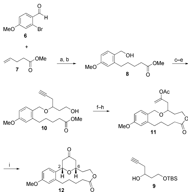
Scheme 3. Substrate synthesis and cyclization: a) 9-BBN, THF, [Pd(dppf)Cl 2 ], K 2 CO 3 , DMF, 50 °C; [10] b) NaBH 4 , MeOH, 50 % (two steps); c) Cl 3 CCN, DBU, CH 2 Cl 2 , 90%; d) 9 , La(OTf) 3 , toluene; [11] e) p -TsOH, MeOH, 60 % (two steps); f) LiOH, THF, MeOH, H 2 O; g) trichlorobenzoyl chloride, Et 3 N, DMAP, toluene, 65 °C, 75 % (two steps); [12] h) HOAc, Na 2 CO 3 , [{Ru( p -cymene)Cl 2 ] 2 }, 1-decyne, toluene, 80 °C, 75 %; [13] i) DDQ, 2,6-dichloropyridine, DCE, 2 h, 73 %. 9-BBN = 9-borabicyclo[3.3.1]nonane, DBU = 1,8-diazabicyclo[5.4.0]undec-7-ene, DCE = 1,2-dichloroethane, DMAP = 4-dimethylaminopyridine, DMF = N,N -dimethylformamide, dppf = 1,1'-bis(diphenylphosphanyl)-ferrocene, TBS = tert -butyldimethylsilyl, Tf = trifluoromethanesulfonyl, Ts = p -toluenesulfonyl.
